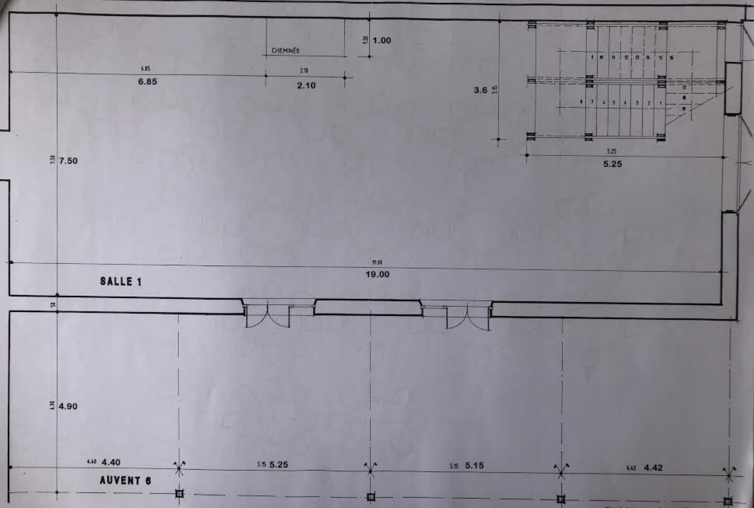
PLAN de SALLE 2cm. = 1m.
